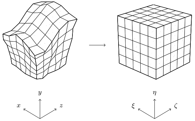
Figure 1. Map of Cartesian space to logical space
