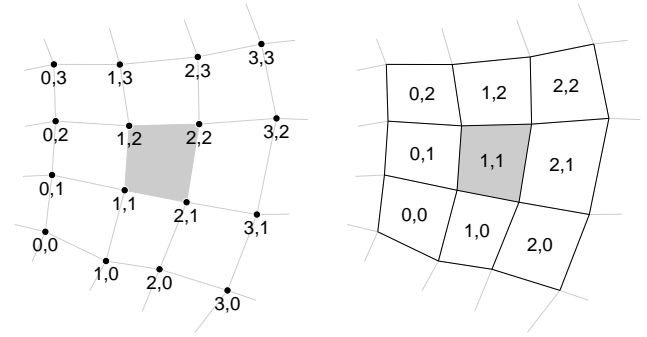
Figure 2. Stencil node and cell indexing for cubic ( n = 3 ) interpolation in the shaded cell (1,1). For simplicity only two dimensions are shown instead of three.
